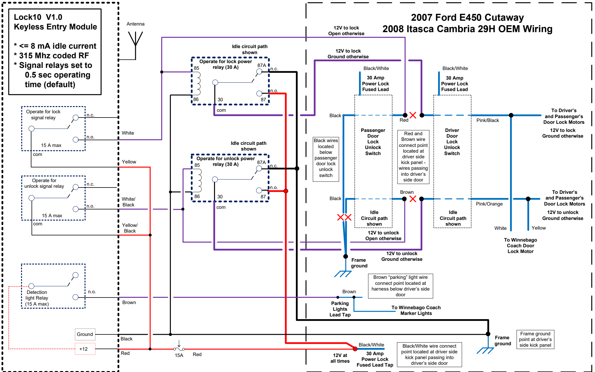
MOTOR COACH MODIFICATION DIAGRAM Keyless Entry Module plus 30 Amp Power Relays 2007 Model Year E450 Super Duty Cutaway 2008 Model Year Itasca Cambria 29H
