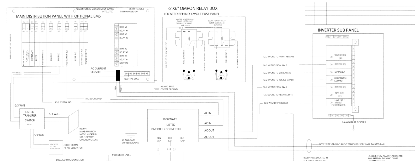
Typical 50 Amp power distribution layout
