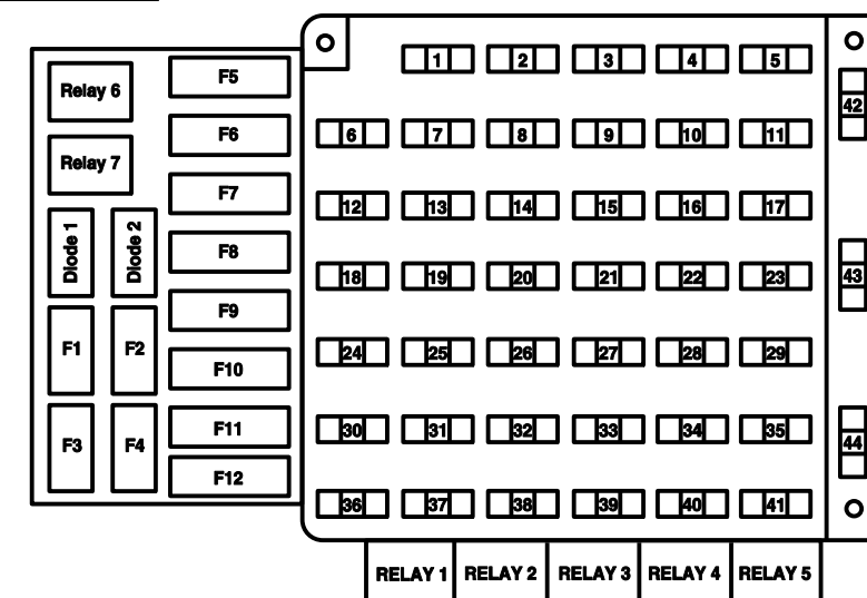
FUSE PANEL
